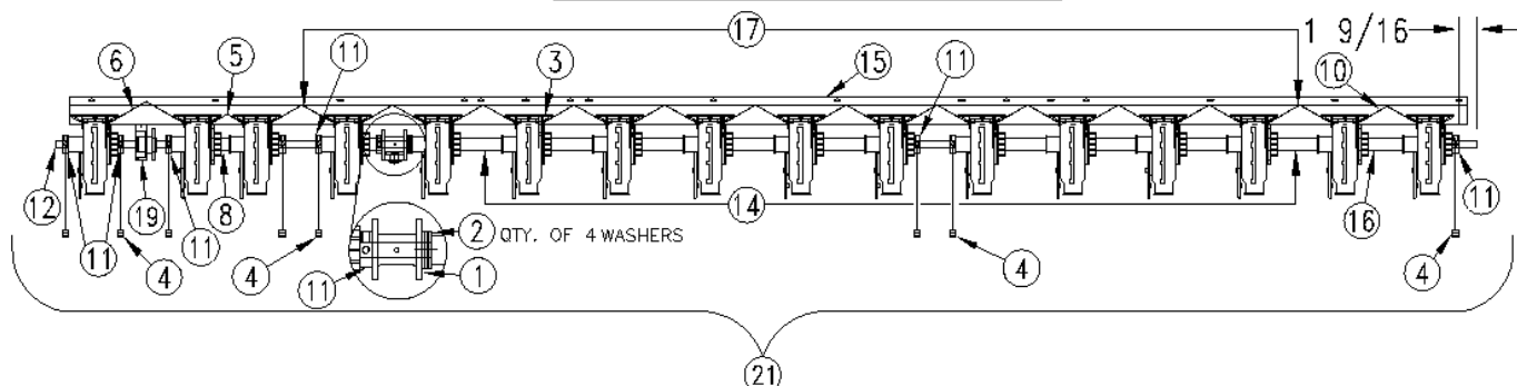
20' - 7.5" LEFT HAND
