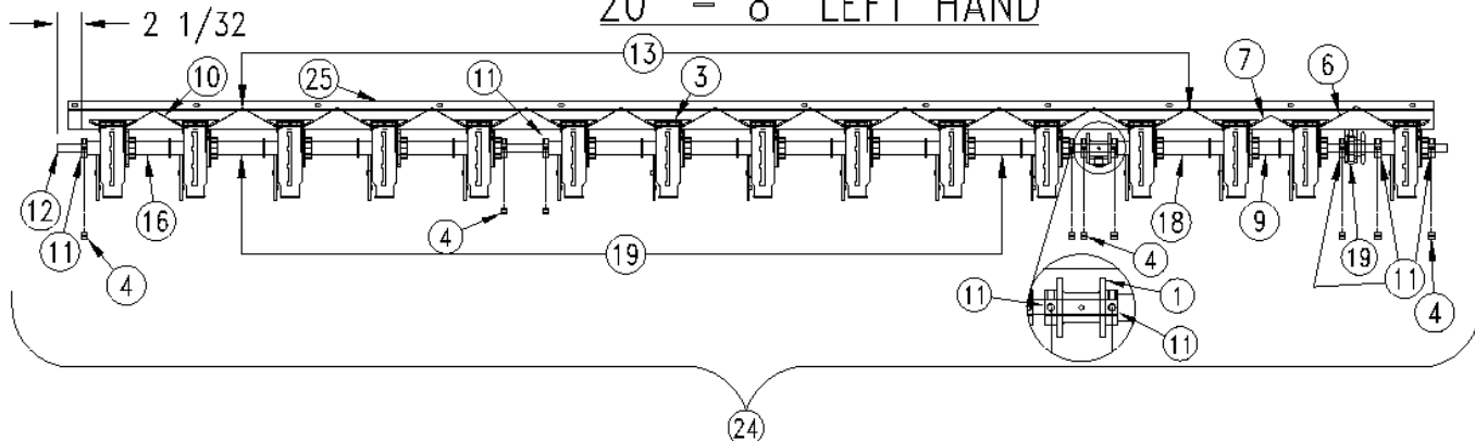
20' - 8" LEFT HAND
