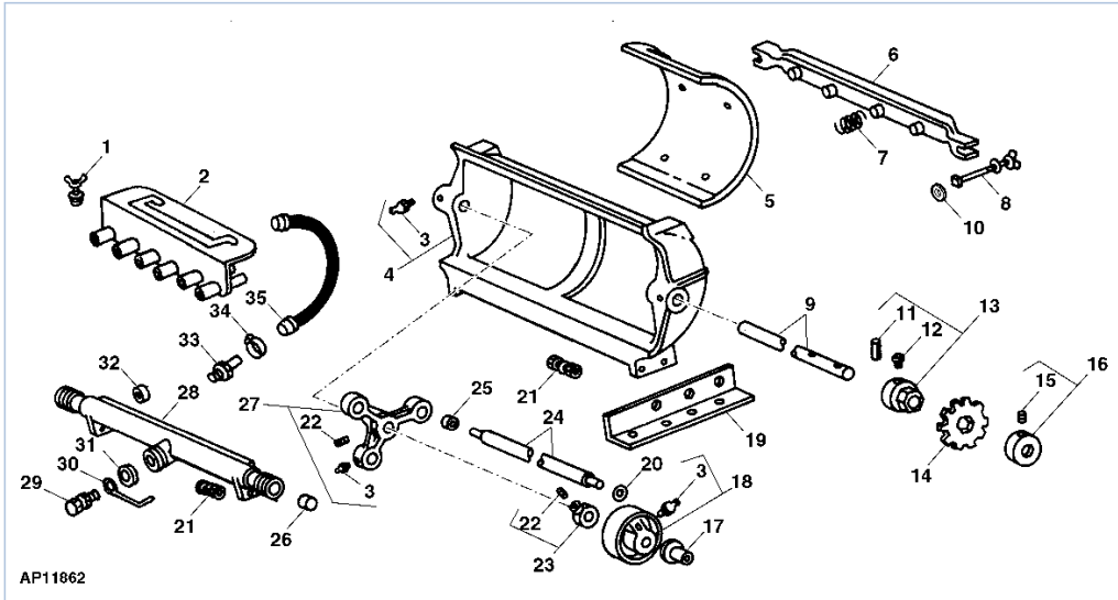
PC1467 150-18 7000 Drawn Cotton and Corn Planter / LIQUID FERTILIZER METERING PUMP (12 ROW NARROW) [H09] PC1467 - HARV-SEEDING
