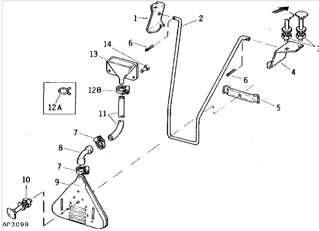
PC1467 160-10 7000 Drawn Cotton and Corn Planter / HERBICIDE DIFFUSER ATTACHMENT (1979-1979) [117] PC1467 - HARV-SEEDING
