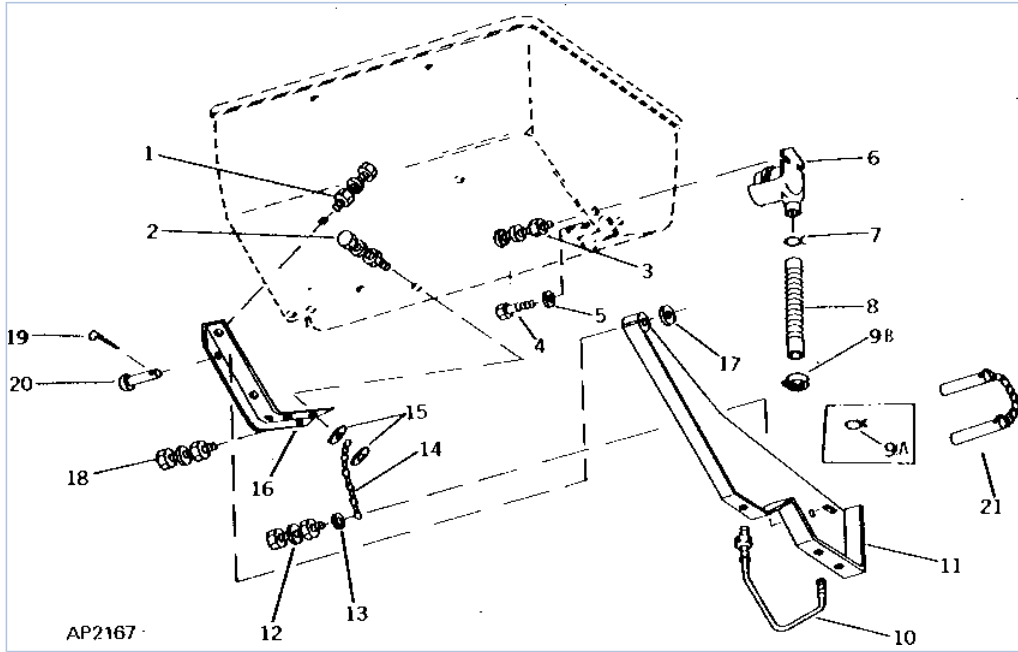
PC1467 150-5 7000 Drawn Cotton and Corn Planter / DRY FERTILIZER HOPPER SUPPORTS AND SPOUTS [G20] PC1467 - HARV-SEEDING
