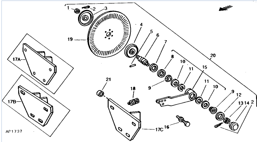
PC1467 110-38 7000 Drawn Cotton and Corn Planter / HEAVY-DUTY COULTER ATTACHMENT (1977-1980) [F15] PC1467 - HARV-SEEDING
