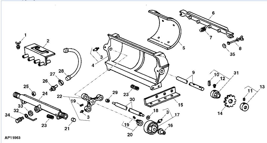
PC1467 150-16 7000 Drawn Cotton and Corn Planter / LIQUID FERTILIZER METERING PUMP (8 ROW NARROW AND 8 ROW WIDE) [H07] PC1467 - HARV-SEEDING
