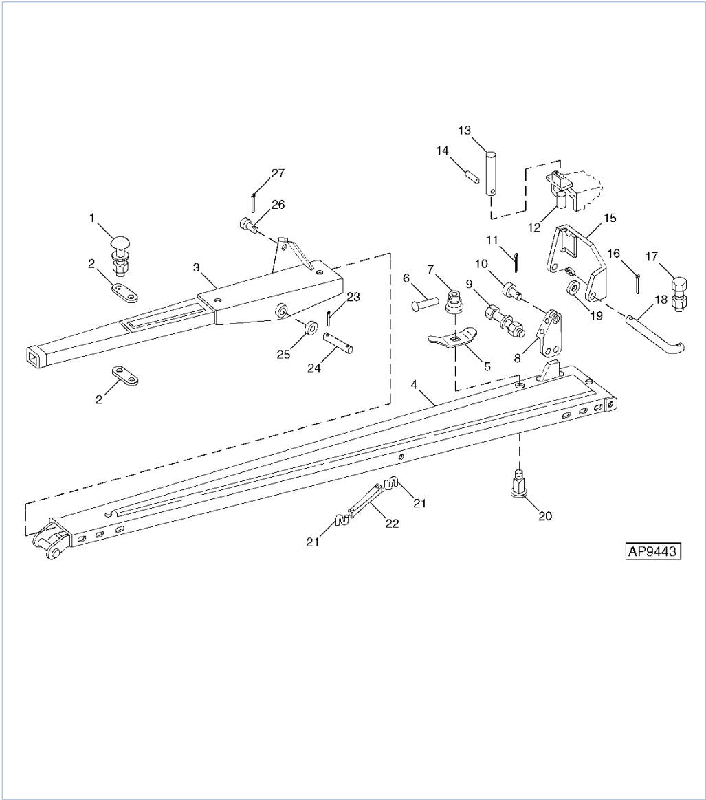
PC1467 120-8 7000 Drawn Cotton and Corn Planter / FOLDING MARKER (8R WIDE AND 12R NARROW) [G08] PC1467 - HARV-SEEDING
