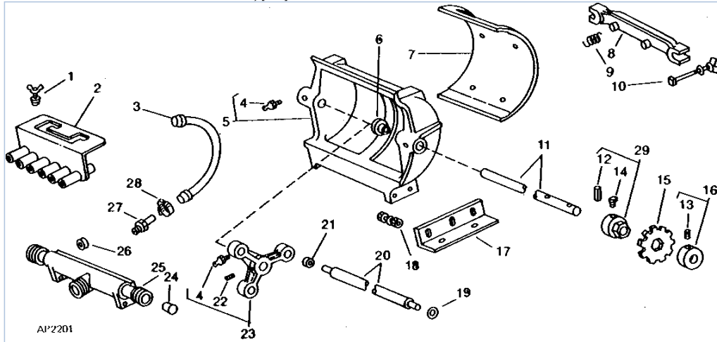
PC1467 150-14 7000 Drawn Cotton and Corn Planter / LIQUID FERTILIZER METERING PUMP (4 ROW NARROW, 4 ROW WIDE, 6 ROW NARROW AND 6 ROW WIDE) [H05] PC1467 - HARV-SEEDING
