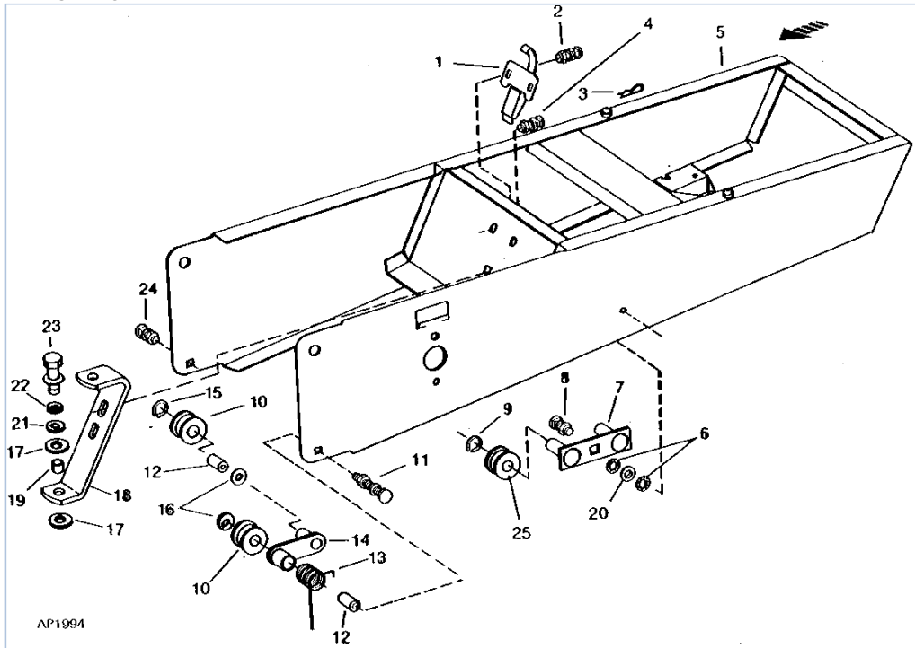
PC1467 110-18 7000 Drawn Cotton and Corn Planter / SUPPORT PANEL AND DRIVE CHAIN TIGHTENER [E21] PC1467 - HARV-SEEDING
