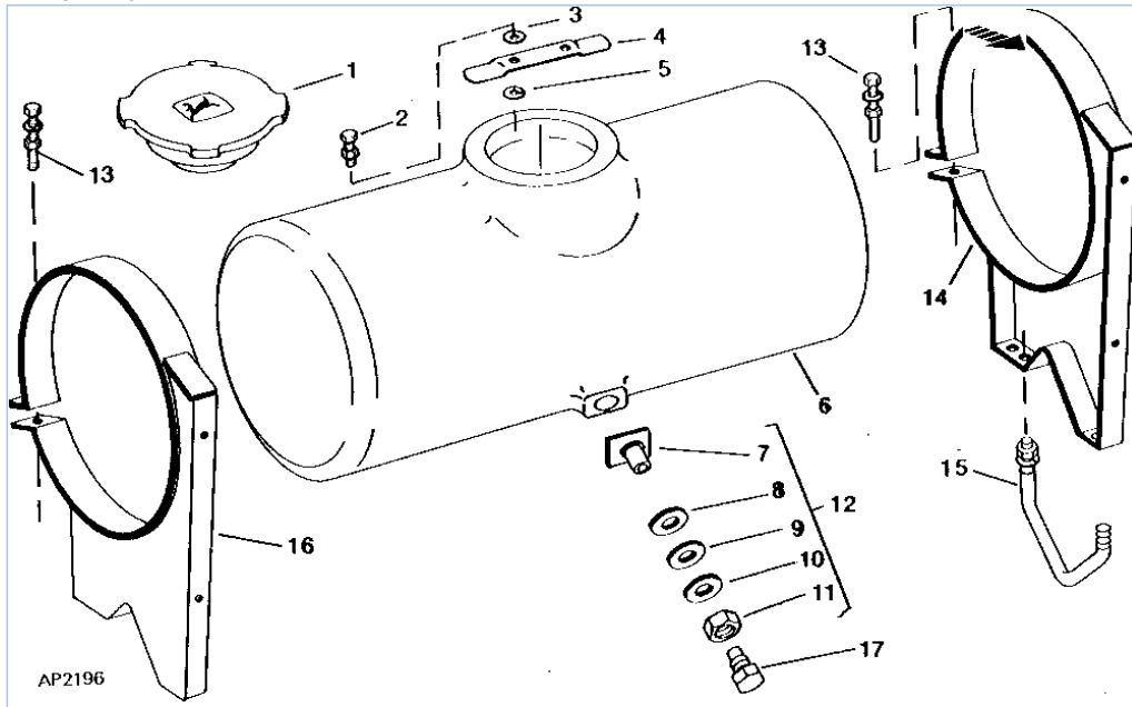
PC1467 150-24 7000 Drawn Cotton and Corn Planter / LIQUID FERTILIZER TANK (-1979)(70 GALLON) [H15] PC1467 - HARV-SEEDING
