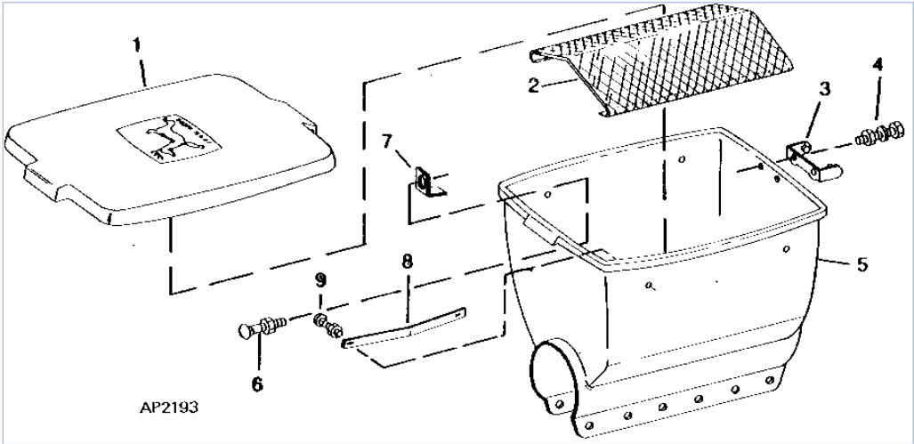
PC1467 150-1 7000 Drawn Cotton and Corn Planter / DRY FERTILIZER AUGER FILL HOPPER [G16] PC1467 - HARV-SEEDING
