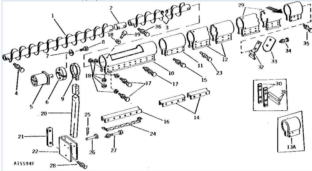
PC1467 150-8 7000 Drawn Cotton and Corn Planter / DRY FERTILIZER AUGER FILL ATTACHMENT (4 ROW NARROW, 4 ROW WIDE AND 6 ROW NARROW) [G23] PC1467 - HARV-SEEDING
