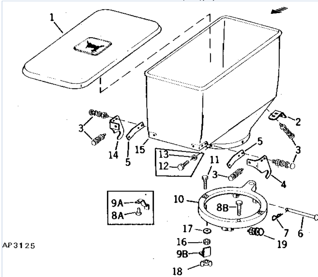
PC1467 110-22 7000 Drawn Cotton and Corn Planter / SEED HOPPER (PLATE) [E25] PC1467 - HARV-SEEDING
