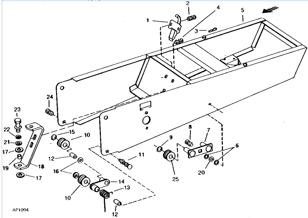
PC1467 160-14 7000 Drawn Cotton and Corn Planter / HOPPER SUPPORT PANEL AND DRIVE CHAIN TIGHTENER (SEED, HERBICIDE, AND INSECTICIDE) [I21] PC1467 - HARV-SEEDING
