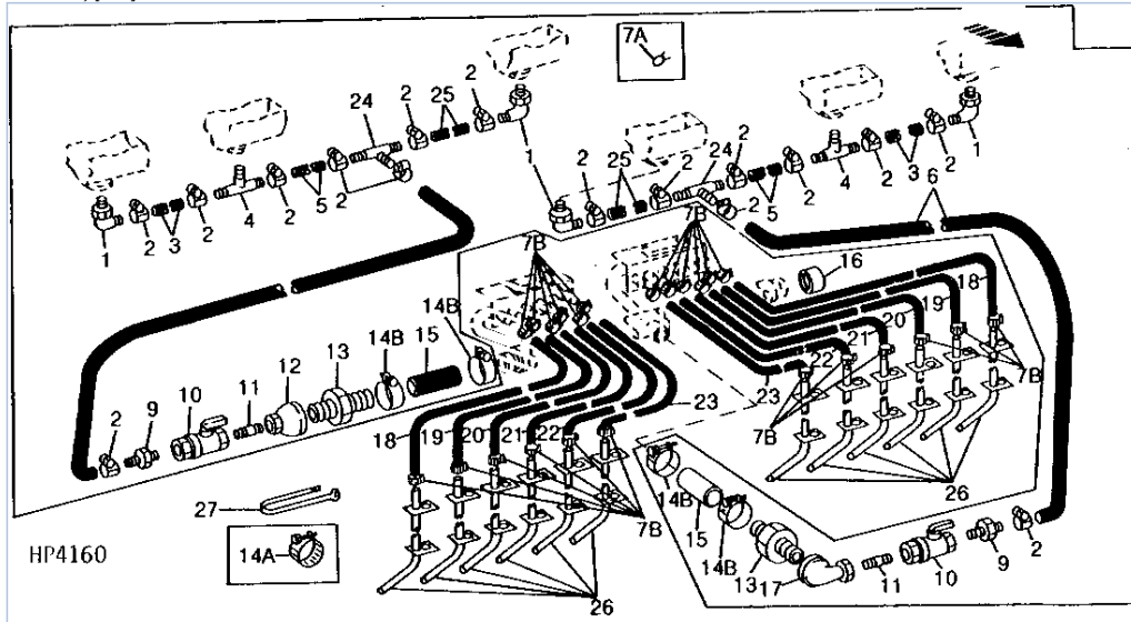
PC1467 150-22 7000 Drawn Cotton and Corn Planter / LIQUID FERTILIZER HOSES, CLAMPS AND FITTINGS (12 ROW NARROW) [H13] PC1467 - HARV-SEEDING
