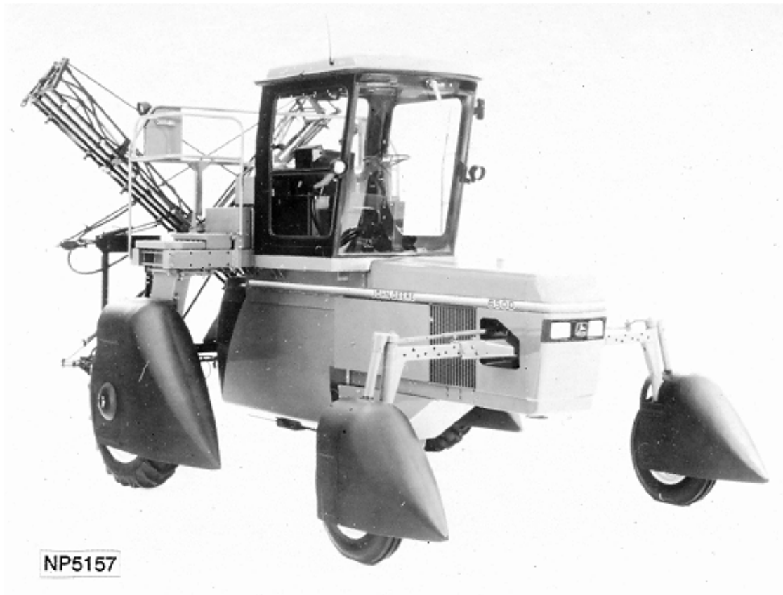
JOHN DEERE 6500 SELF-PROPELLED SPRAYER WIDE FRONT, WITH SOUND GARD® CAB AND 60-FOOT BOOM (MANUFACTURED 1993- )
